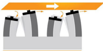
3 The second pair now extends and repositions on the rod. Their tips move right. The first pair retracts and their tips bend left.
