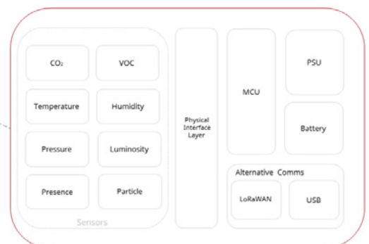
Sensor Node - Block Diagram
